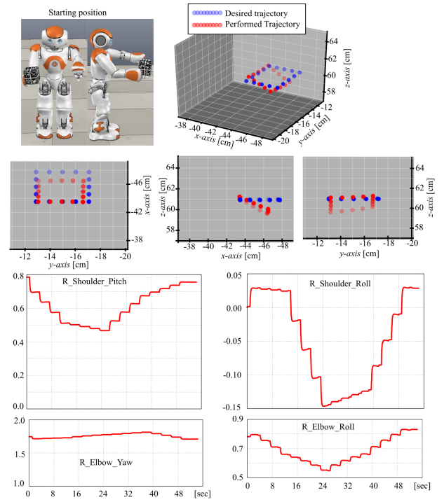
Fig. 7: The end-effector moves along a 4 [cm] \times 4 [cm] square shape in X-Y plane (Left \rightarrow Forward \rightarrow Right \rightarrow Backward) with fixed orientation in Cartesian space. The starting configurations of the right arm are ShoulderPitch 45°, ShoulderRoll 0°, ElbowYaw 100°, ElbowRoll 45°, WristYaw 0°.
