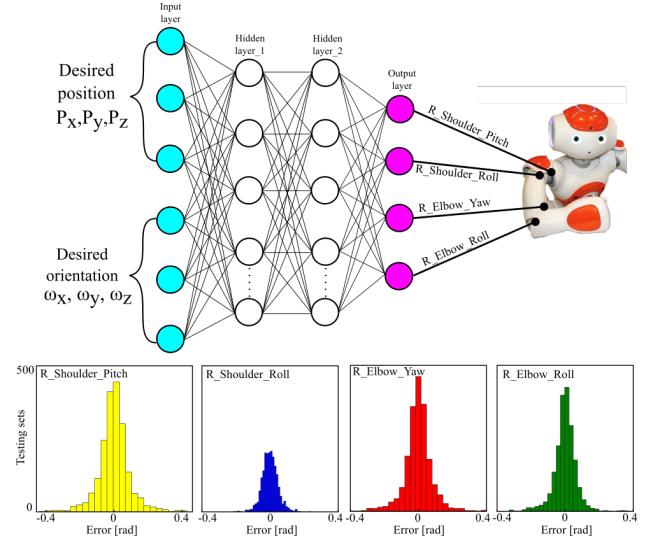
Fig. 3: Inverse model neural network, two hidden layers with 25 neurons each layer, one input layer with 6 input neurons and one output layer with 4 output neurons (top). Histograms of the error of inverse kinematics based on the neural network representation (bottom).
