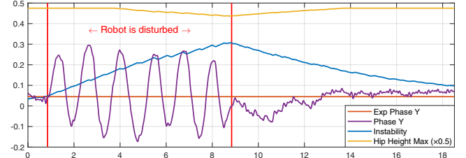
(c) Oscillations in the robot orientation, induced artificially here, cause the calculated instability to increase and limit the maximum allowed hip height.
