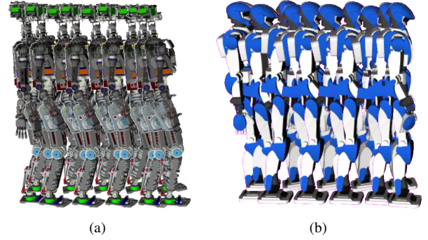
Fig. 5: Execution of a post-processed sequence of stances only allowing foot contacts on (a) ARMAR-4 and (b) HRP-4.
