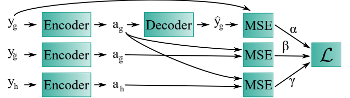
Fig. 3: For training the network is provided with three samples at the same time to define the loss function
