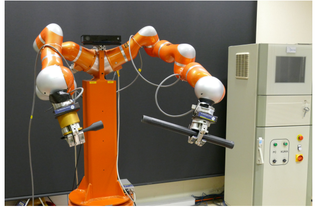
Fig. 5. Experimental setup
