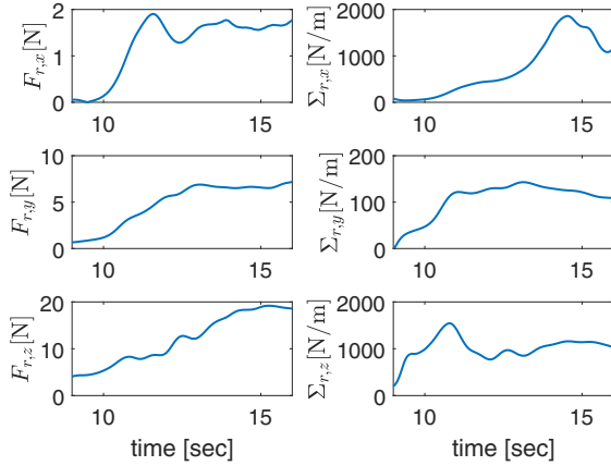
Fig. 7. Measure relative forces and estimated relative stiffness during the relative peg-in-hole operation. Relative direction y is in the direction of the peg insertion, where the robot estimated low stiffness. Note also that the initially estimated stiffness in x coordinate was also low, as the interaction forces in this direction were initially very low.
